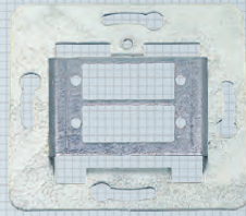
Module mounting plate, 2-fold SC-Duplex
