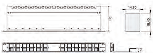
Cut-out dimensions Keystone cut-out
