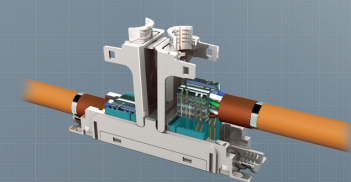
preLink® Extender Cat. 6 A ISO/IEC CKEA0100 (Solid Version)
