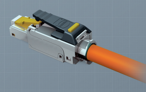
preLink® RJ45 Connector module Cat. 6 A ISO/IEC CKSA0100
