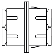
SC-Duplex, Grade C
